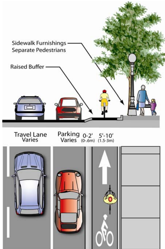
Figure 2. Example Section Design for Cycle track with On-Street Parking
