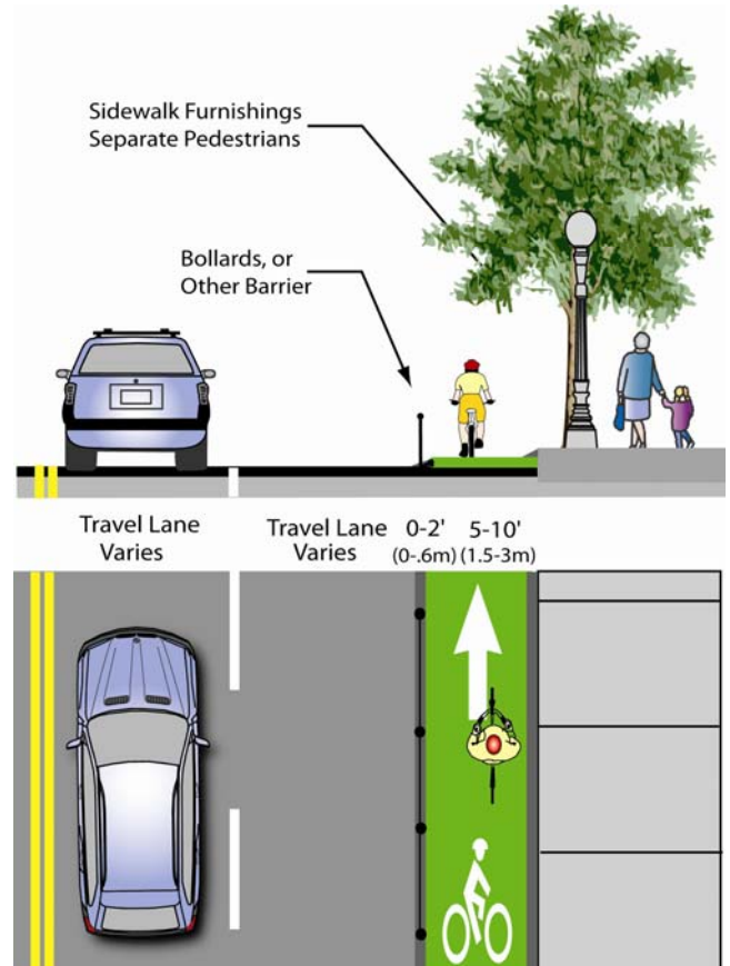
Figure 3. Example Section Design of a Cycle track without Parking
