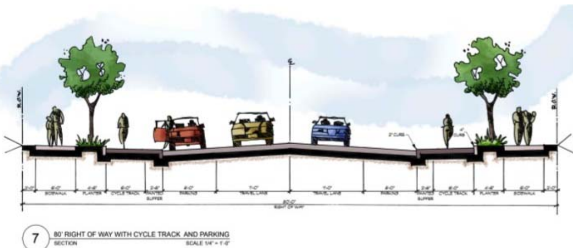
Figure 26. Cross-Section for Cully Boulevard Cycle Track in Portland, OR
